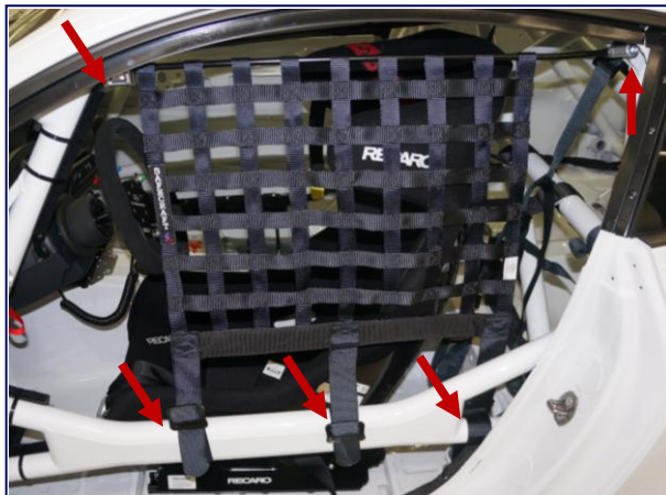
Driver Window Net Mounting Points
