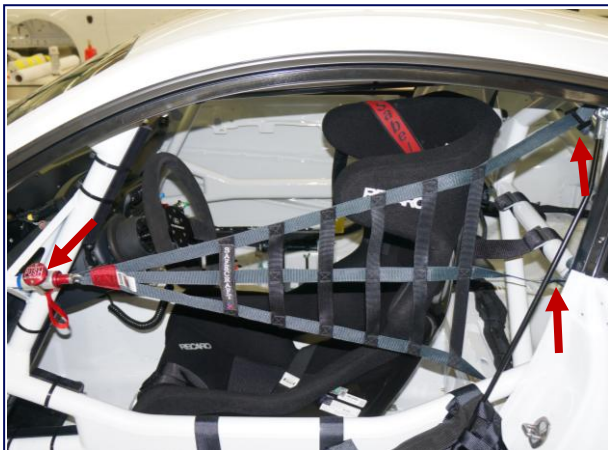
Driver Helmet Support Net Mounting Points
